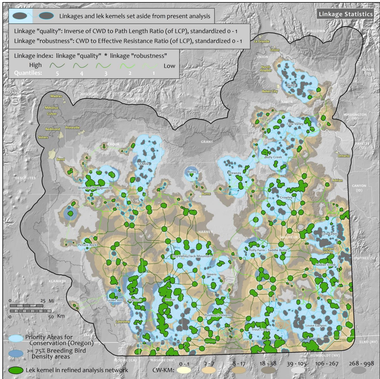
Figure 9: Linkage Statistics
