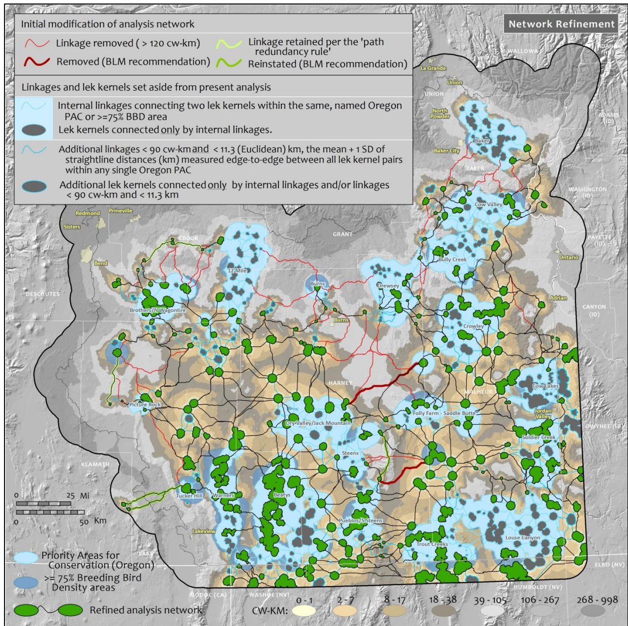
Figure 8: Network Refinement
